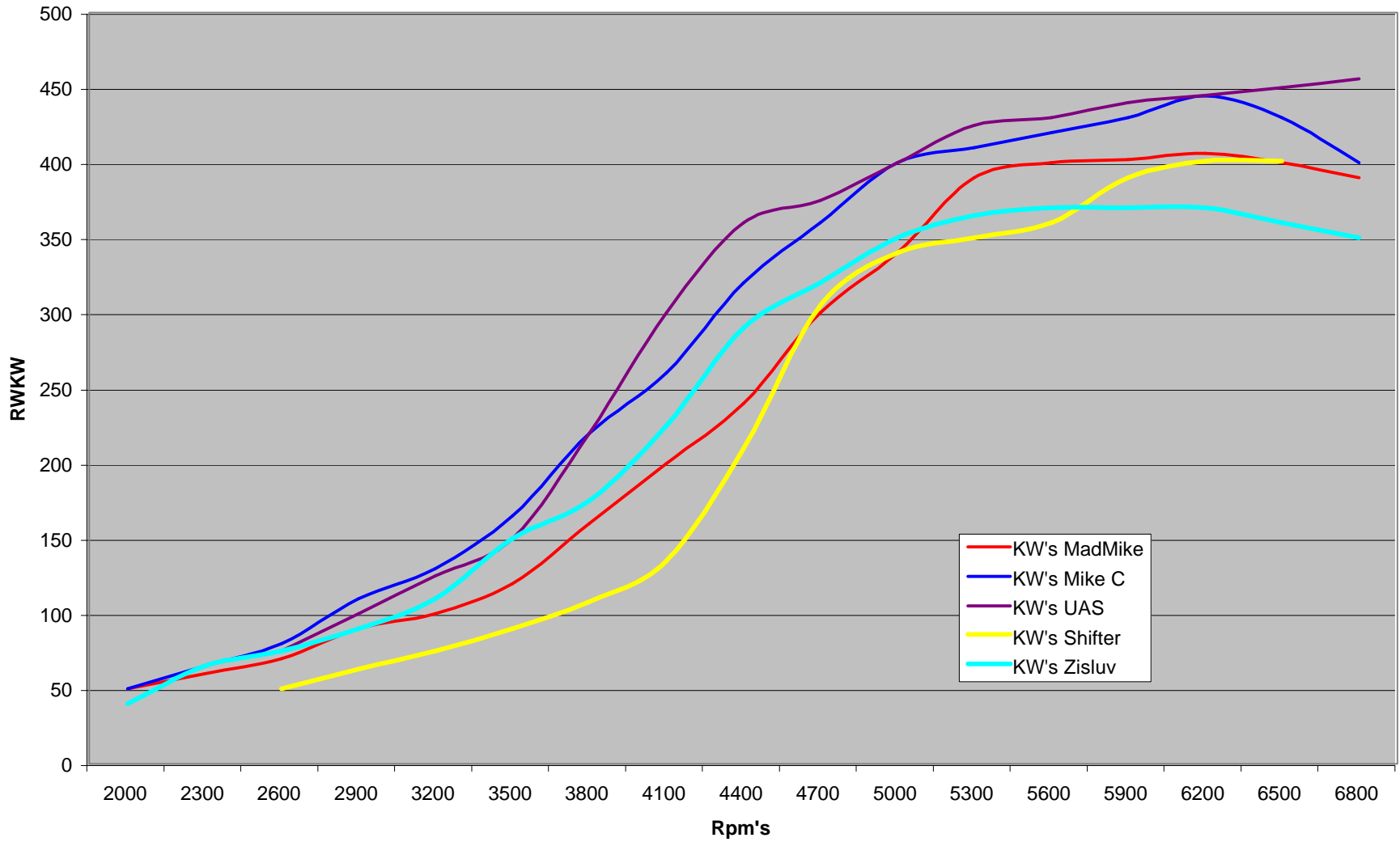
Dyno Comparison
