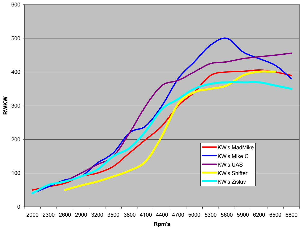
Dyno Comparison
